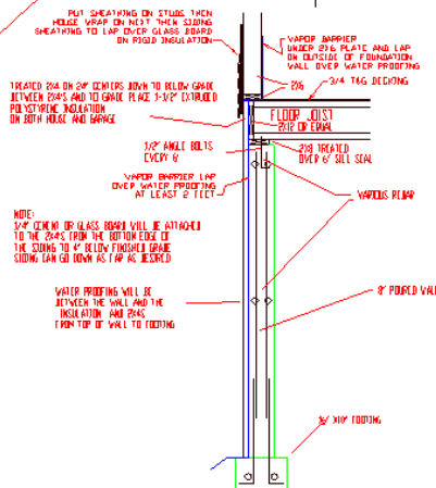
POURED WALL DETAIL
